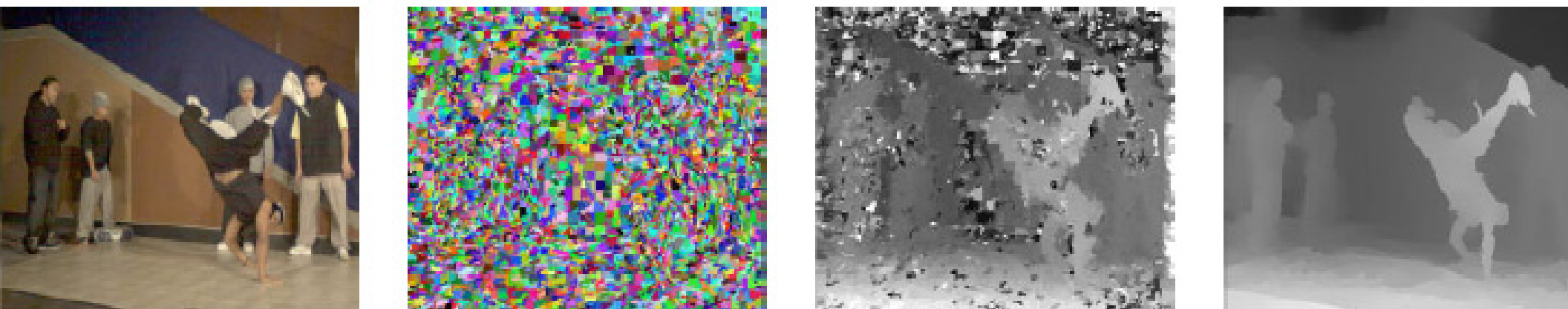
Segmentation-based stereo matching (Zitnick, Kang, Uyttendaele et al. 2004) c 2004 ACM: (a) input color image; (b) color-based segmentation; (c) initial disparity estimates; (d) final piecewise-smoothed disparities;
