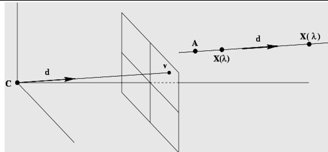
Fig. 8.14. Vanishing point formation. (a) Plane to line camera. The points X_i, i = 1, \dots, 4 are equally spaced on the world line, but their spacing on the image line monotonically decreases. In the limit X \rightarrow \infty the world point is imaged at x = v on the vertical image line, and at x = v on the inclined image line. Thus the vanishing point of the world line is obtained by intersecting the image plane with a ray parallel to the world line through the camera centre C . (b) 3-space to plane camera. The vanishing point, v , of a line with direction d is the intersection of the image plane with a ray parallel to d through C . The world line may be parametrized as X(\lambda) = A + \lambda D , where A is a point on the line, and D = (d^T, 0)^T .
