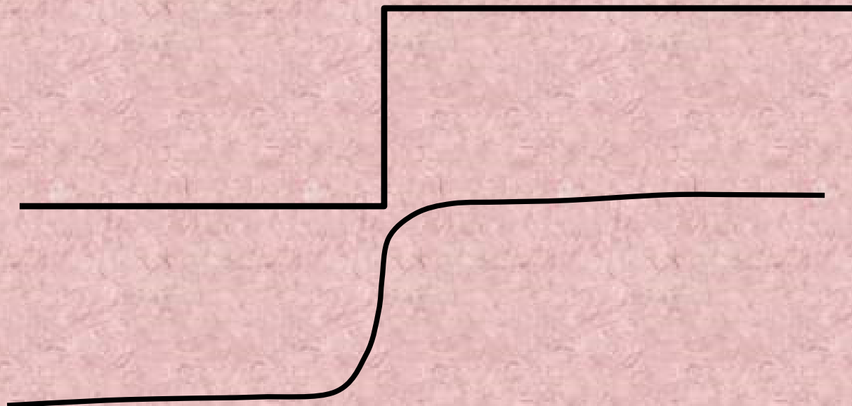
Ideal Step edge in 1-D
