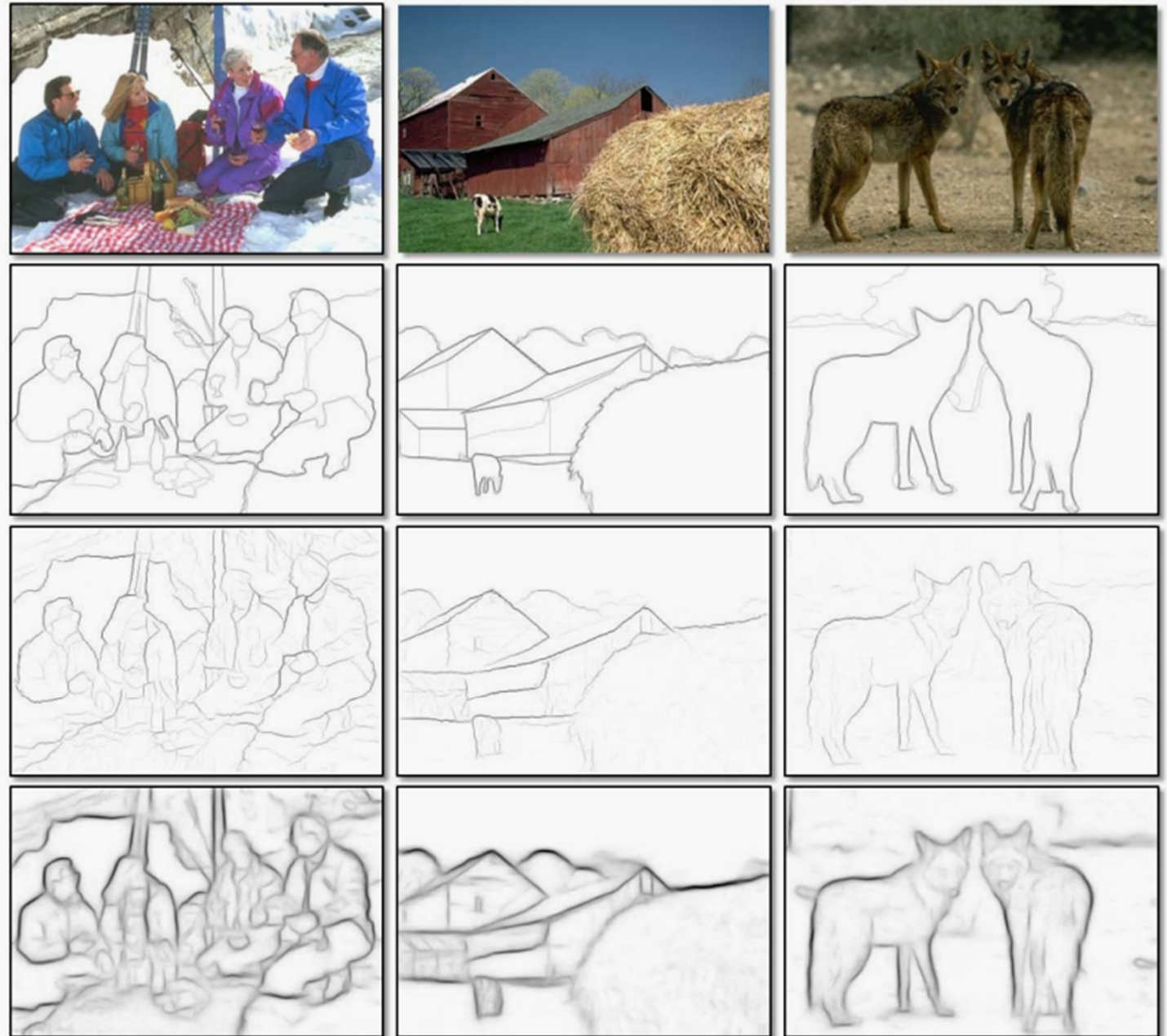
Row 1 - Input Images from BSDS500 Dataset; Row 2 - Ground Truth Row 3 - SCG output ; Row 4 - Structured Edges (SE) – (this work)
