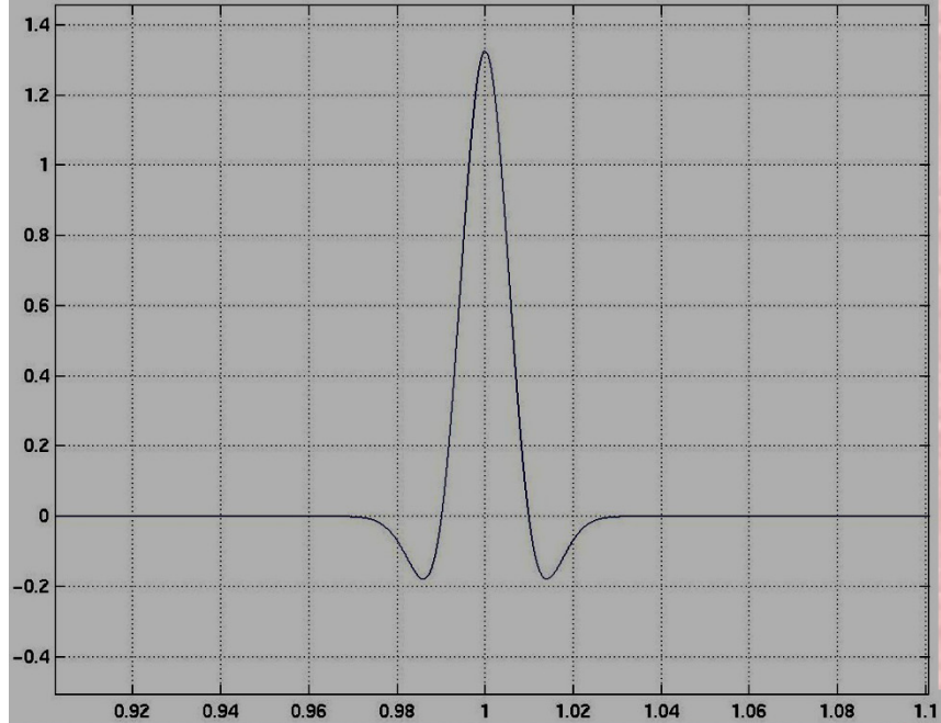
LOG operator in 1-D
