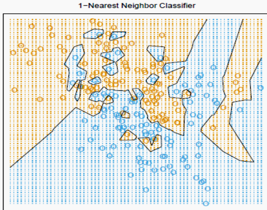
FIGURE 2.3. predicted by 1-nearest-neighbor classification.
