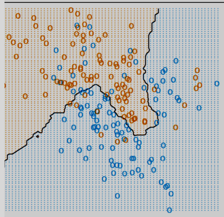
FIGURE 2.2. The same classification example in two dimensions as in Figure 2.1. The classes are coded as a binary variable (BLUE = 0, ORANGE = 1) and then predicted by 15-nearest-neighbor averaging as in (2.8). The predicted class is hence majority vote amongst the 15-nearest neighbors.
