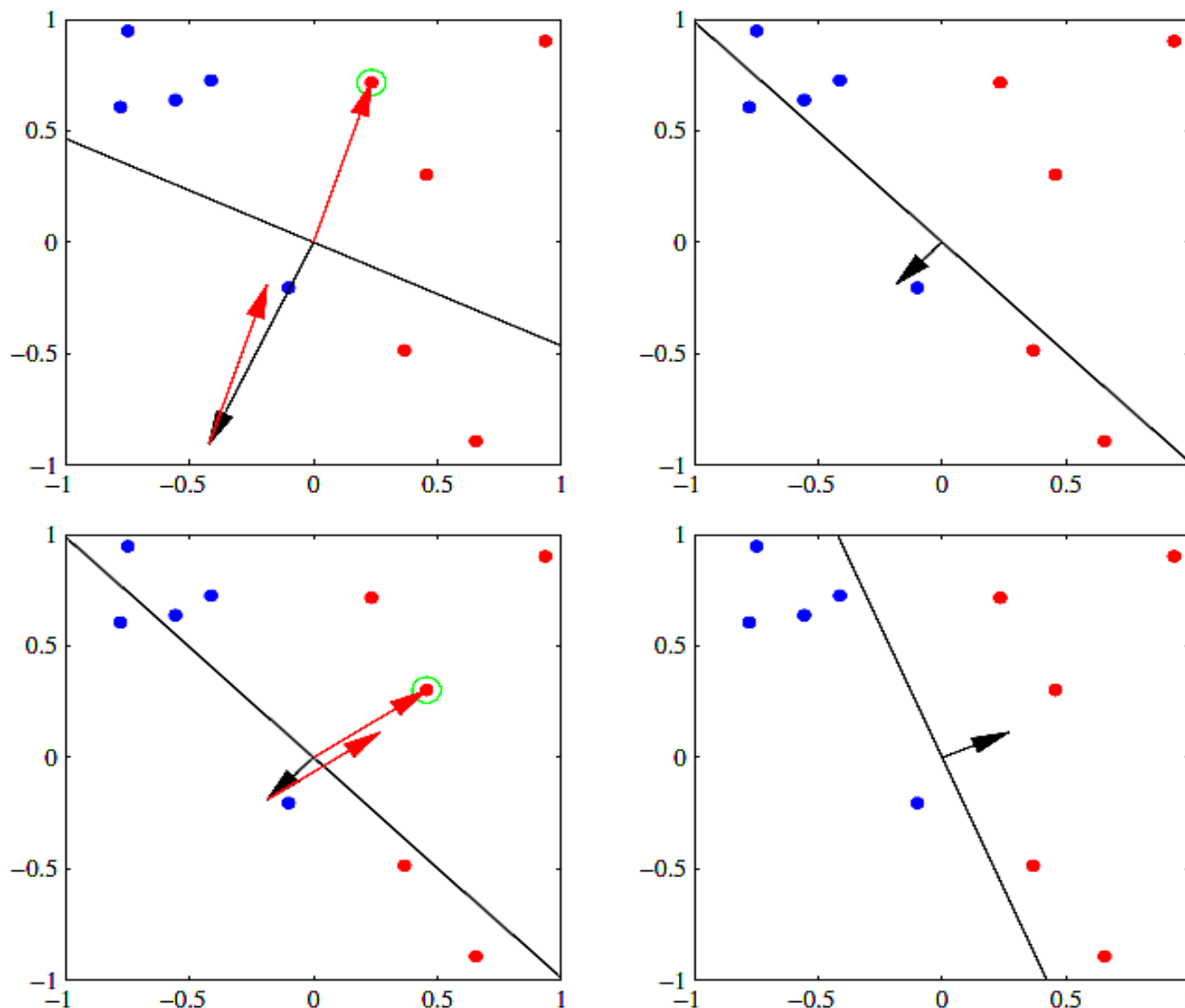
Figure 4.7 Illustration of the convergence of the perceptron learning algorithm, showing data points from two classes (red and blue) in a two-dimensional feature space ( \phi_1, \phi_2 ). The top left plot shows the initial parameter vector w shown as a black arrow together with the corresponding decision boundary (black line), in which the arrow points towards the decision region which classified as belonging to the red class. The data point circled in green is misclassified and so its feature vector is added to the current weight vector, giving the new decision boundary shown in the top right plot. The bottom left plot shows the next misclassified point to be considered, indicated by the green circle, and its feature vector is again added to the weight vector giving the decision boundary shown in the bottom right plot for which all data points are correctly classified.
