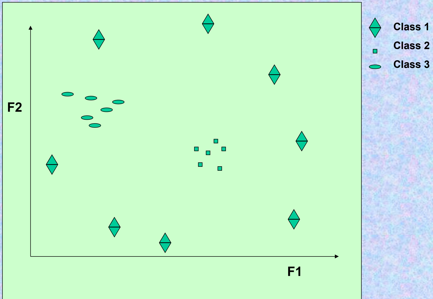
Sample points in a two-dimensional feature space
