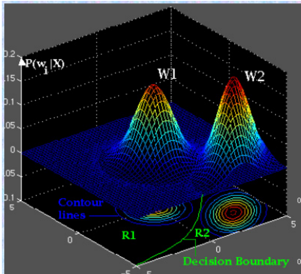
An example of 2-D DRs: R1 and R2; with a non-linear DB.
